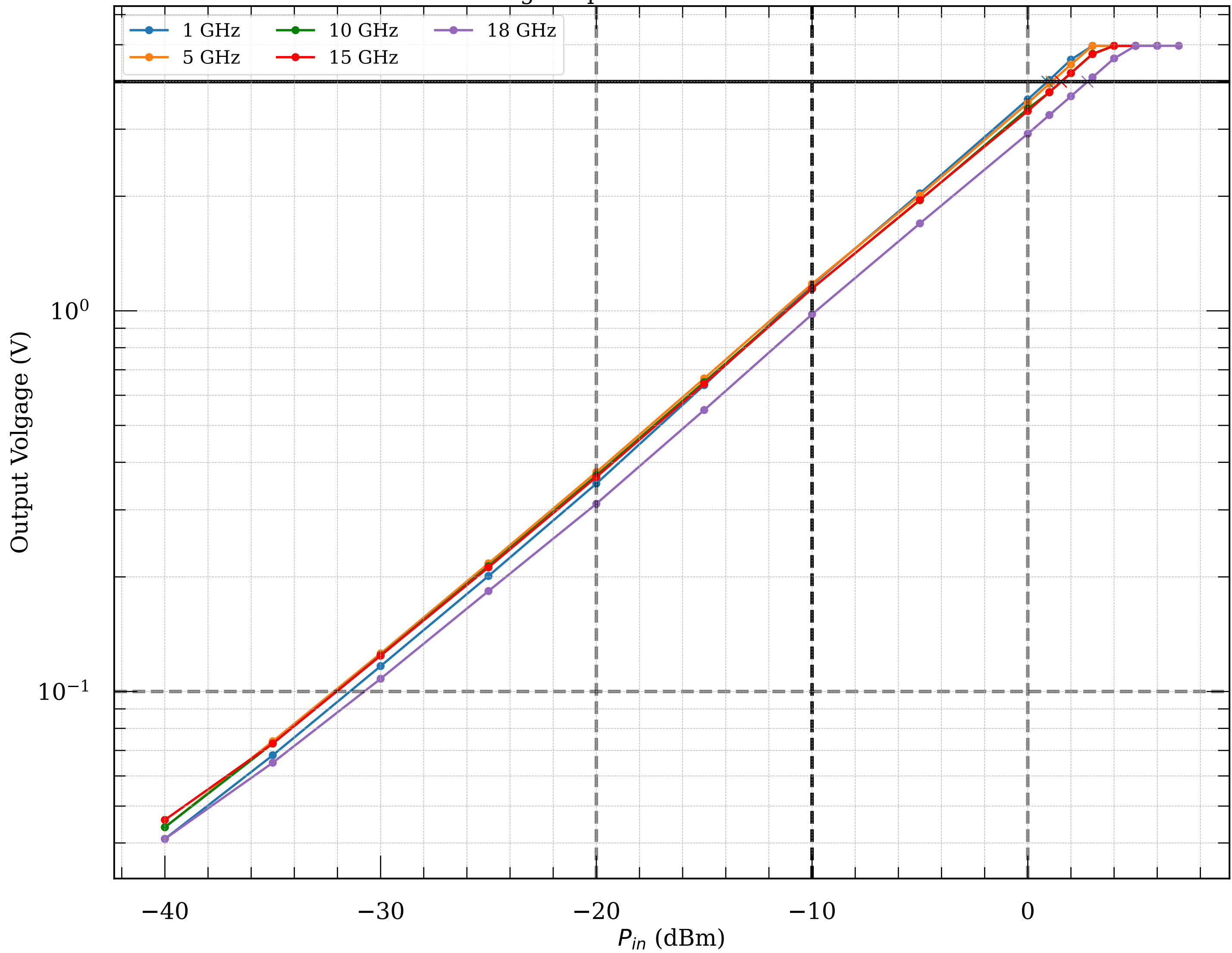
Measured voltage-to-power curve of detector module083
